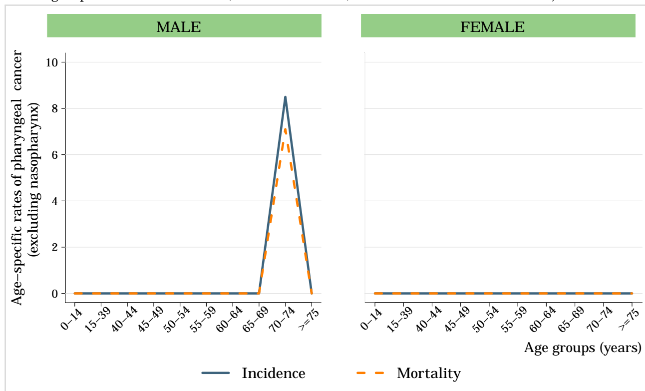
Figure 28: Comparison of incidence and mortality rates of the pharynx (excluding nasopharynx) by age group and sex in Zimbabwe (estimates for 2012). Includes ICD-10 codes: C09-10,C12-14
