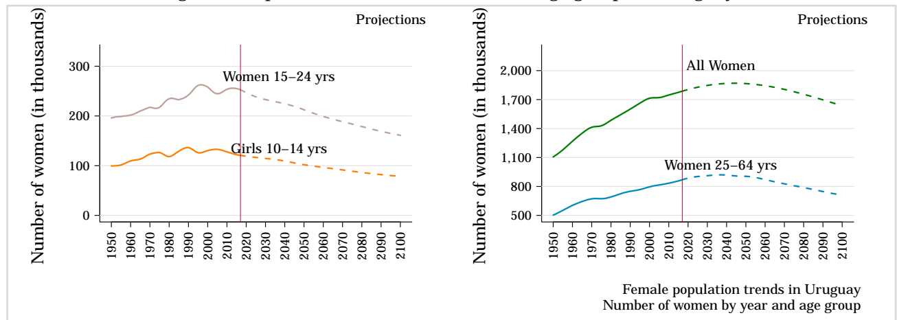
Figure 3: Population trends in four selected age groups in Uruguay
