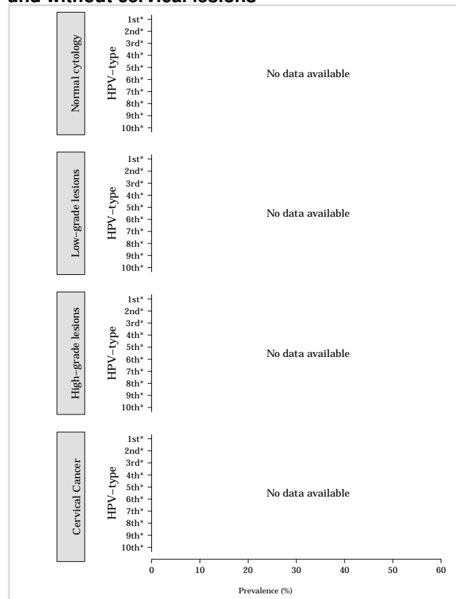
Figure 1. Comparison of the ten most frequent HPV oncogenic types in Grenada among women with and without cervical lesions
