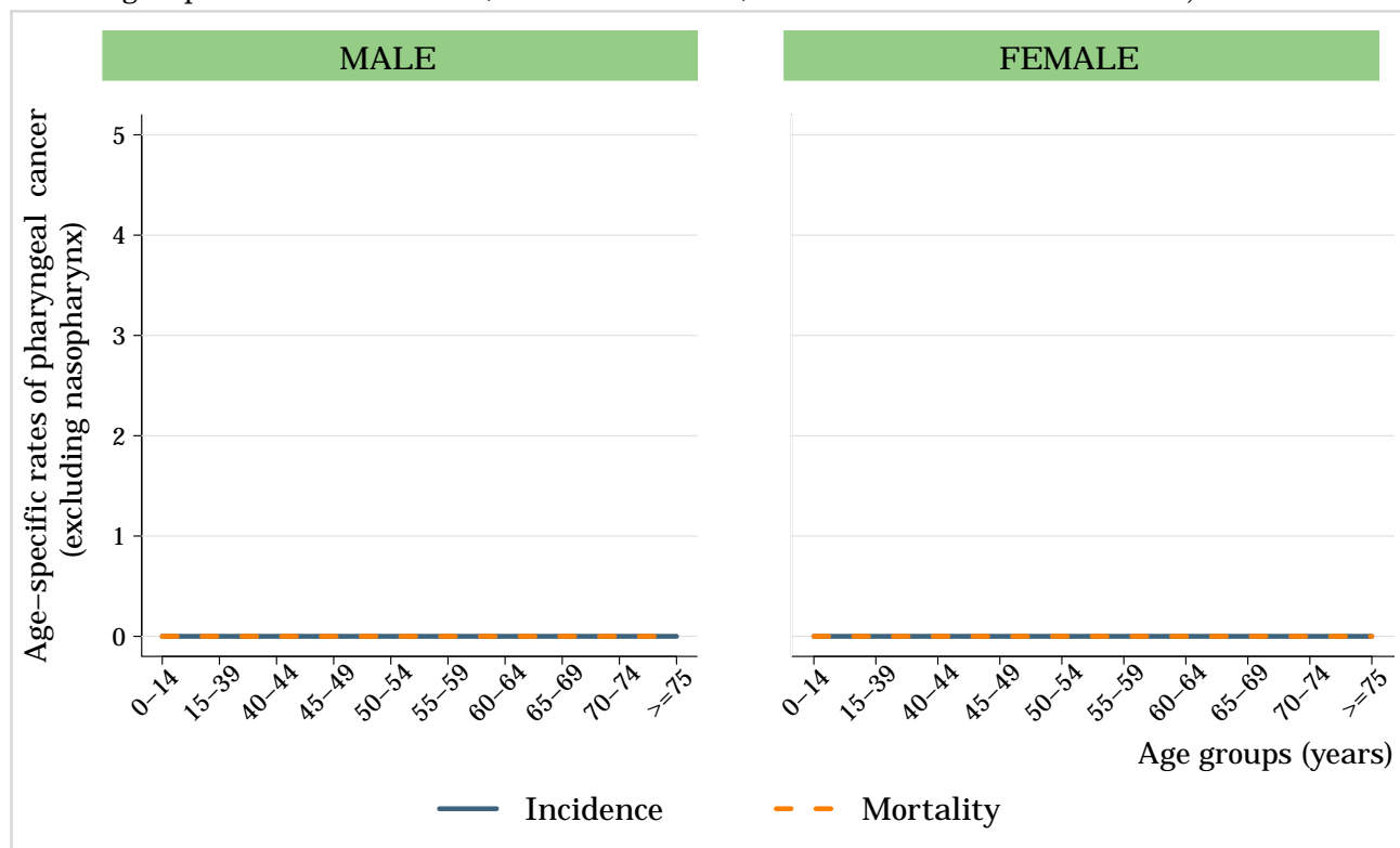
Figure 23: Comparison of incidence and mortality rates of the pharynx (excluding nasopharynx) by age group and sex in Grenada (estimates for 2012). Includes ICD-10 codes: C09-10,C12-14
