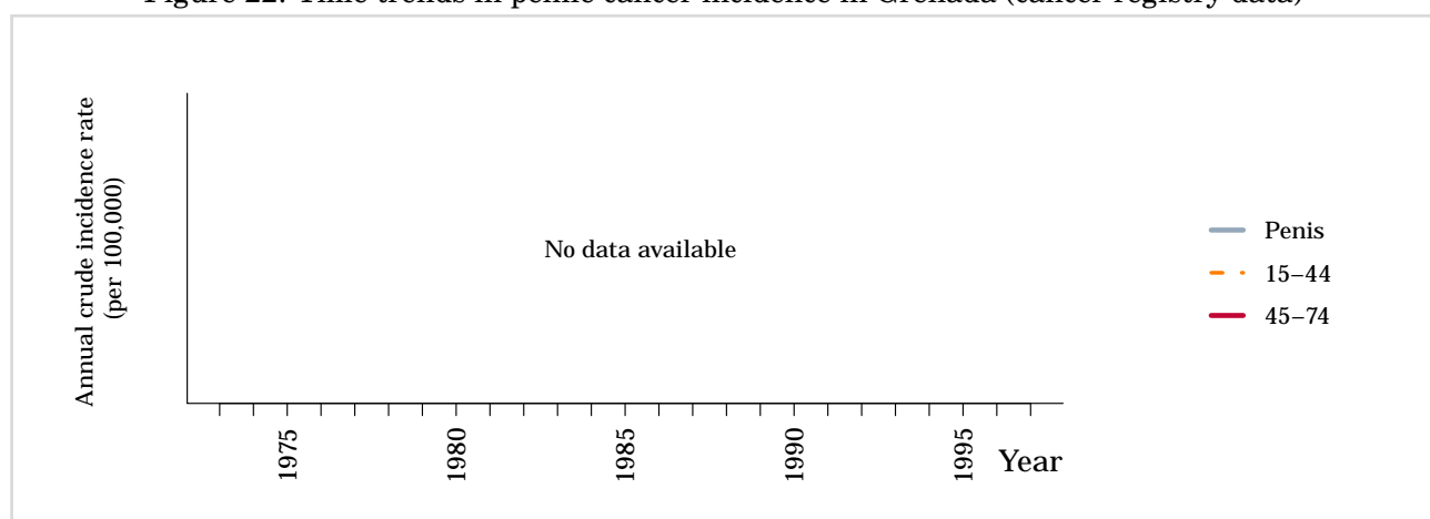
Figure 22: Time trends in penile cancer incidence in Grenada (cancer registry data)
