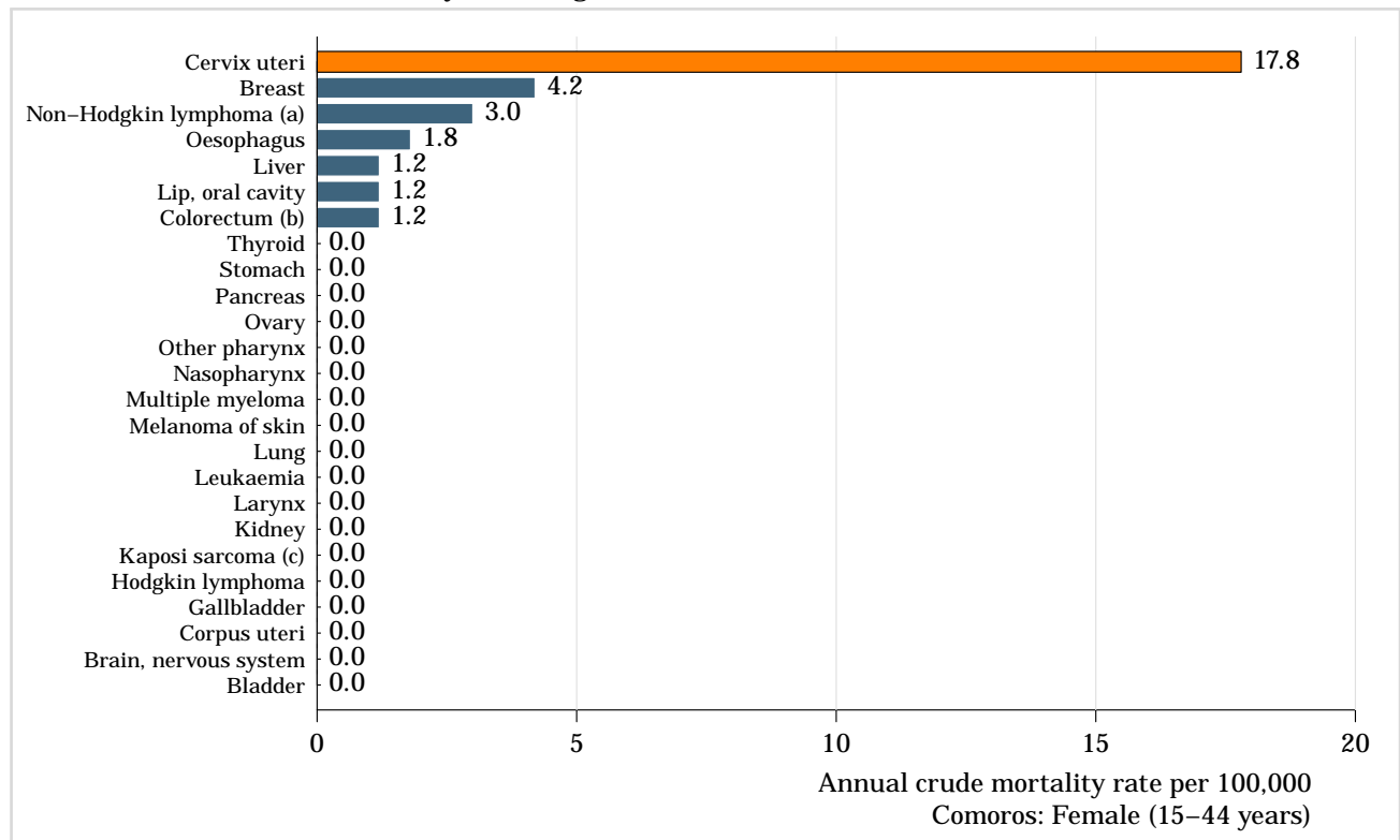
Figure 12: Comparison of age-specific mortality rates of cervical cancer to other cancers among women 15-44 years of age in Comoros (estimates for 2012)
