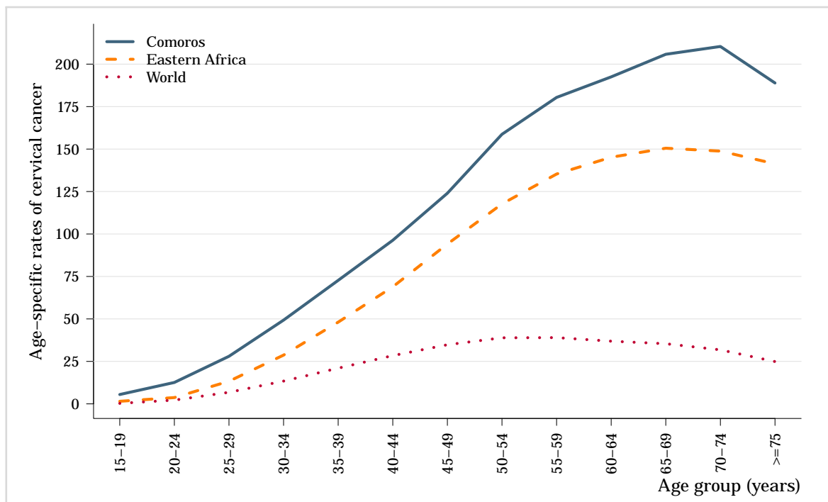
Figure 9: Comparison of age-specific cervical cancer incidence rates in Comoros, within the region, and the rest of world
