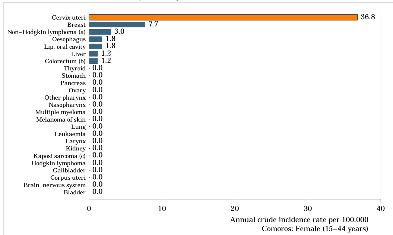
Figure 5: Comparison of age-specific cervical cancer to age-specific incidence of other cancers among women 15-44 years of age in Comoros (estimates for 2012)
